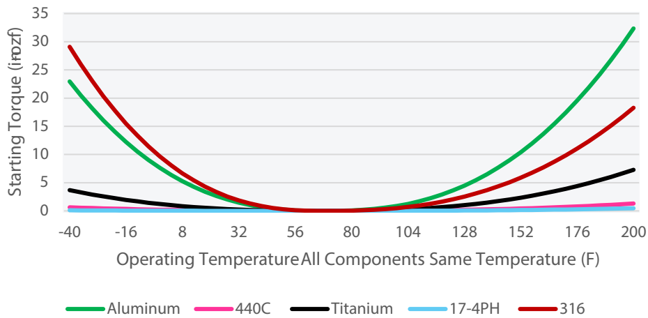
52100 Bearing Rings/Balls, 1/4" Thick Shaft and Housing Wall - Torque by Material
