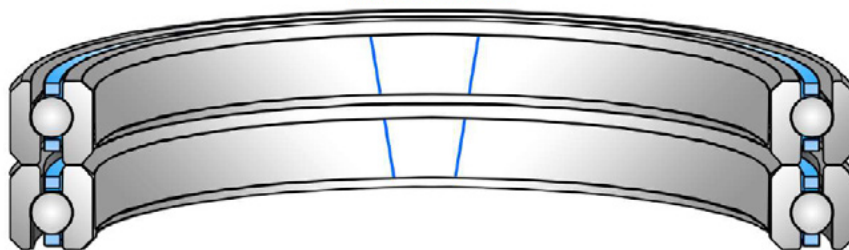
Incorrect Orientation
