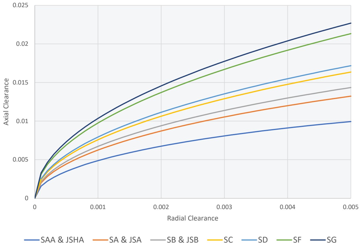
C-Type Radial vs Axial Clearance by Series 1
