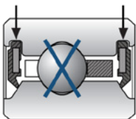
X - TYPE SEALED OR SHIELDED
