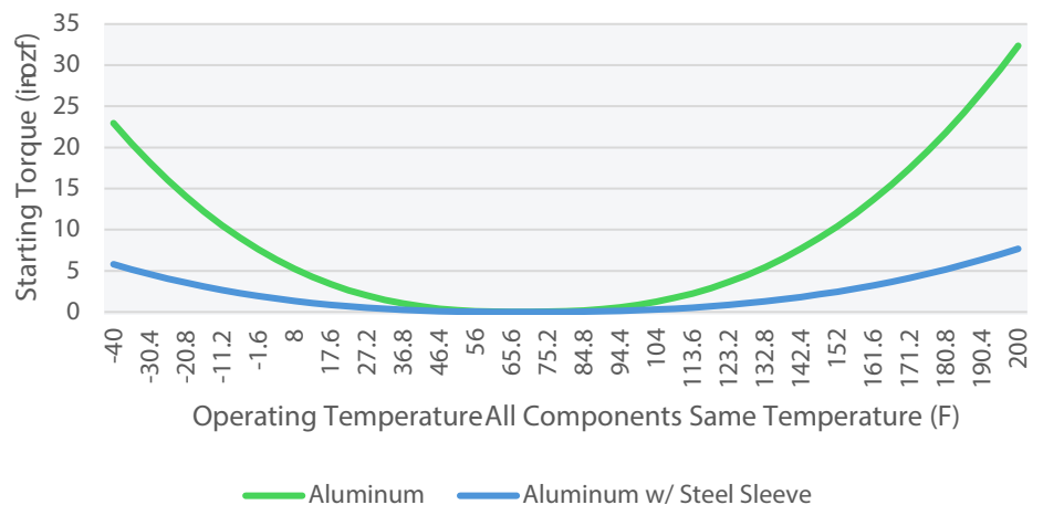
52100 Bearing Rings/Balls, 1/4" Thick Wall Aluminum vs Steel Sleeved Aluminum Shaft and Housing
