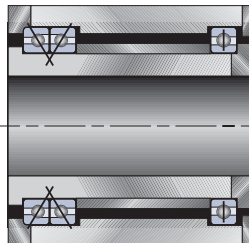
"A" Type "F" pair & floating "C" type mounting
