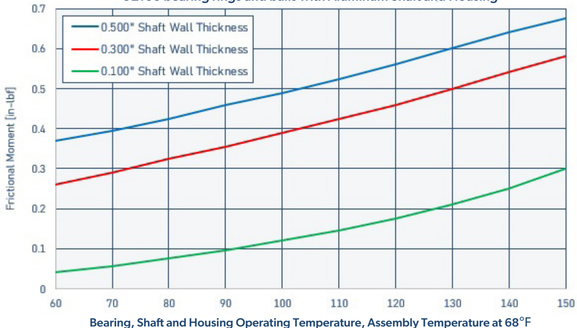
Example of Wall Thickness and CTE Mismatch Effects on Torque 52100 bearing rings and balls with Aluminum Shaft and Housing
