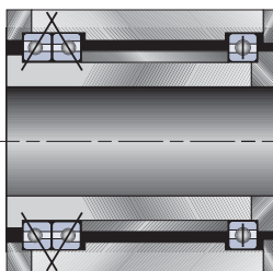
"A" Type "B" pair "C" Type radial thrust floating
