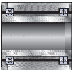
"X" Type & floating "C" Type mounting reversing thrust load & radial loads
