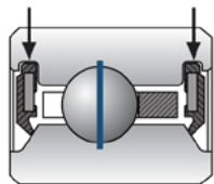
C - TYPE SEALED OR SHIELDED
