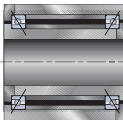
Face-to-Face mounting
