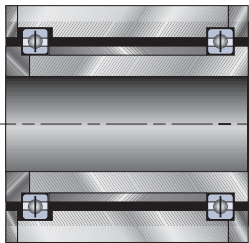
"C" Type radial loading with one floating bearing
