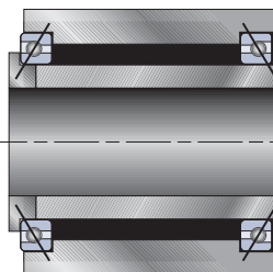
Back-to-Back mounting
