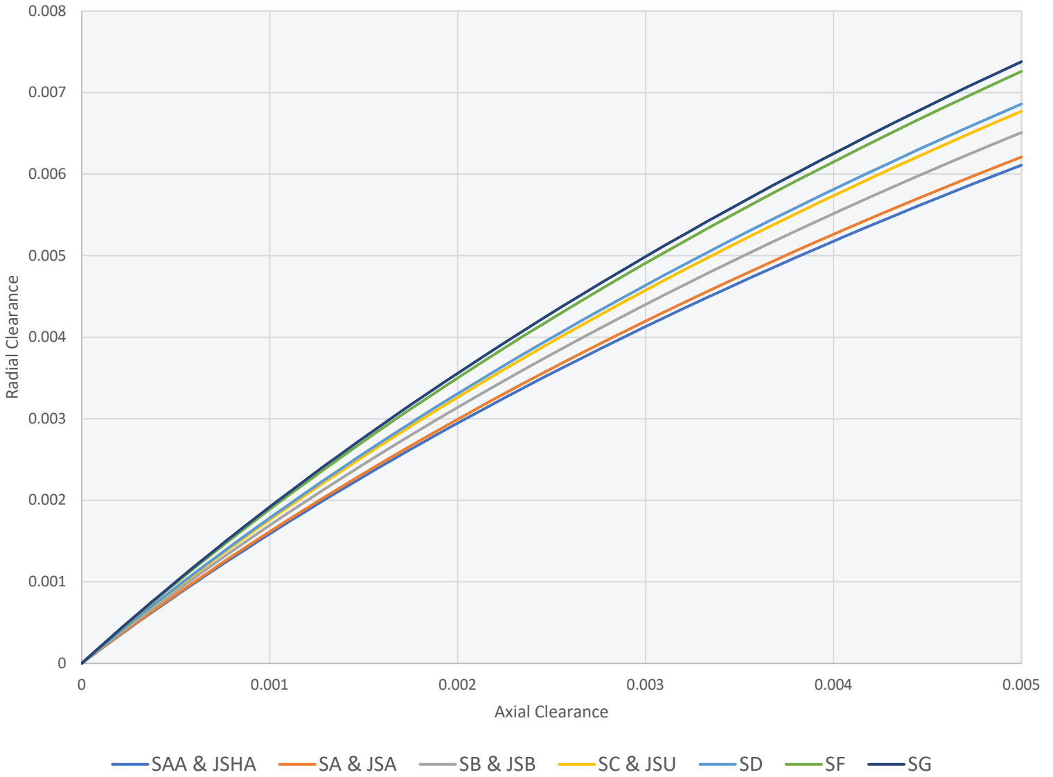
X-Type Radial vs Axial Clearance by Series
